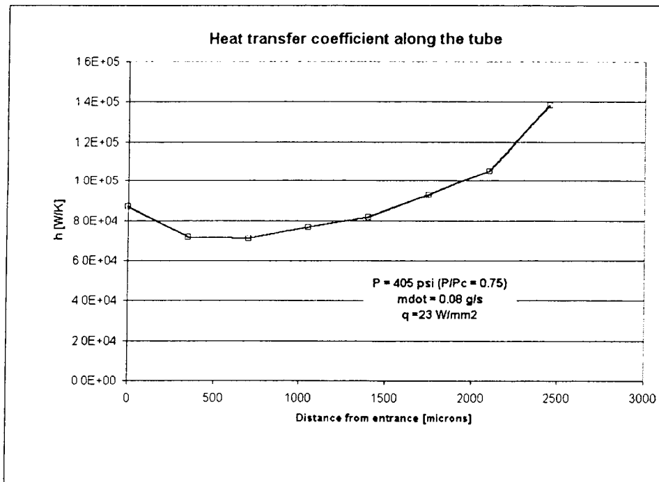
Figure 5-7: Heat transfer coefficient profile for a test with JP10 at a pressure P = 405 psi ( \frac{P}{P_c} = 0.75 ), a mass flow \dot{m} = 0.08 g/s and a heat flux q = 23 W/mm 2 .
