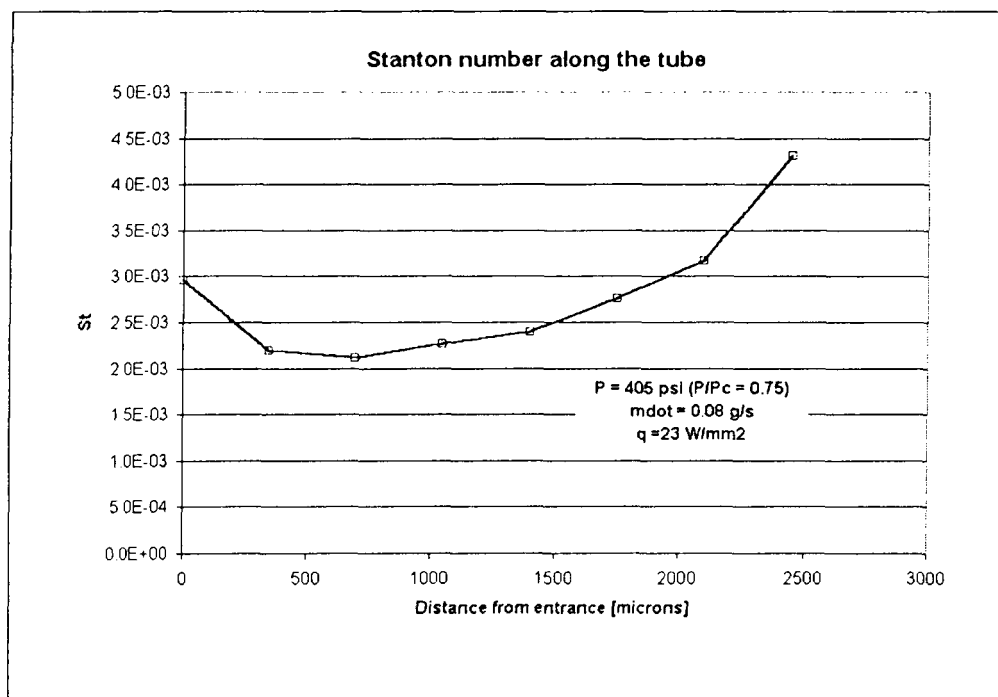
Figure 5-11: Stanton number profile for a test with JP10 at a pressure P = 405 \text{ psi} ( \frac{P}{P_c} = 0.75 ), a mass flow \dot{m} = 0.08 \text{ g/s} and a heat flux q = 23 \text{ W/mm}^2 .
