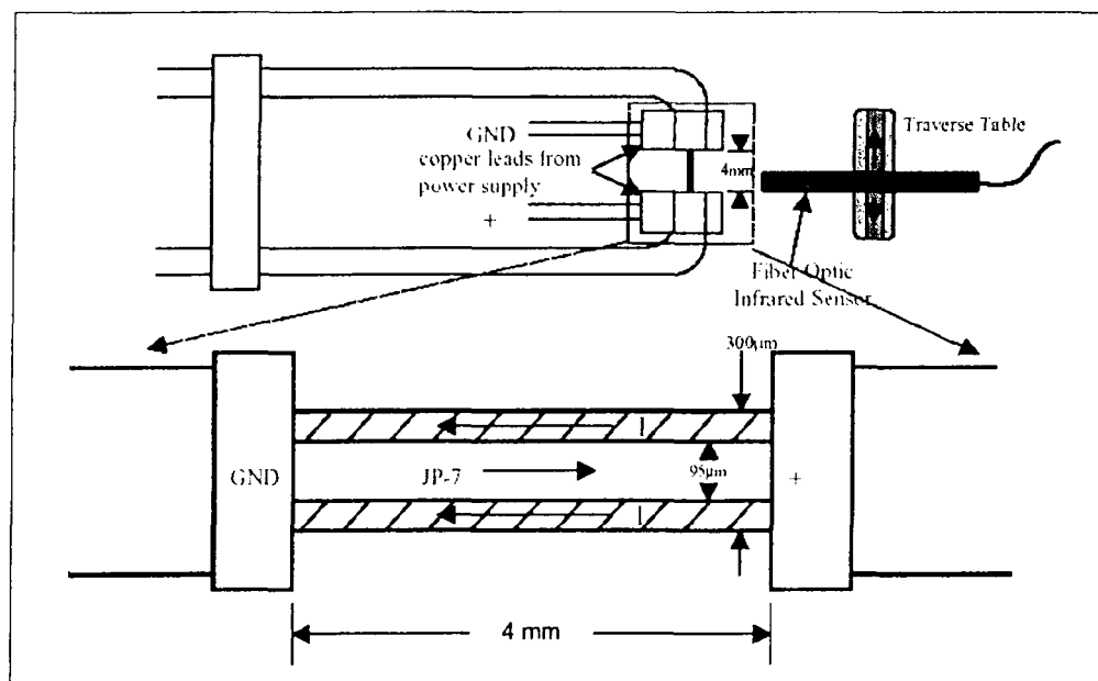
Figure 3-6: Schematic of the test section and the heating system.
