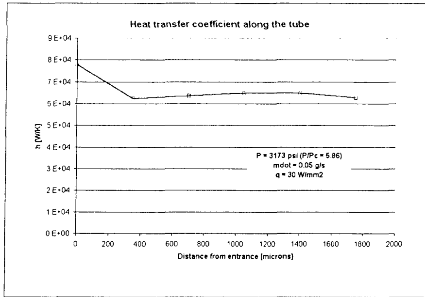
Figure 5-9: Heat transfer coefficient profile along the tube for a test carried out with JP10 at a pressure P = 3,173 \text{ psi} ( \frac{P}{P_c} = 5.86 ), a mass flow \dot{m} = 0.05 \text{ g/s} and a heat flux q = 30 \text{ W/mm}^2 .
