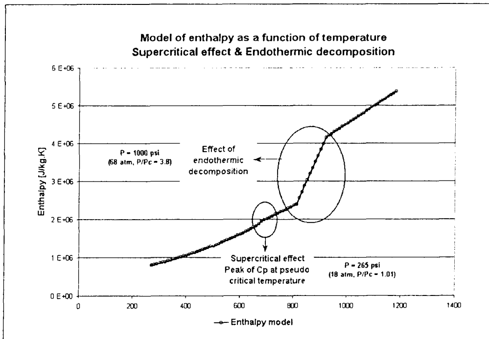
Figure 4-7: Comparison of the effects of both phenomena. The enthalpy profile of JP7 is shown as a function of temperature. The supercritical effect is calculated from the specific heat of JP7 at P=265 psi ( \frac{P}{P_c}=1.01 ). The effect of the endothermic reaction is estimated from experimental data at macro scale at P=1,000 psi.
