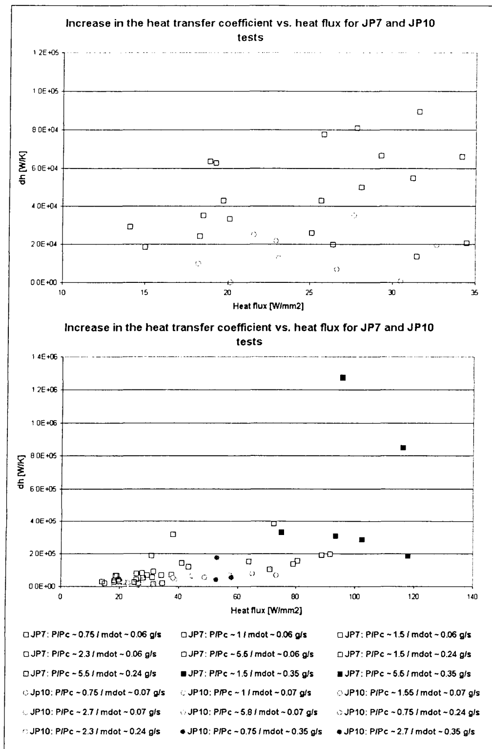
Figure 5-26: Increase in the heat transfer coefficient along the tube as a function of heat flux.
