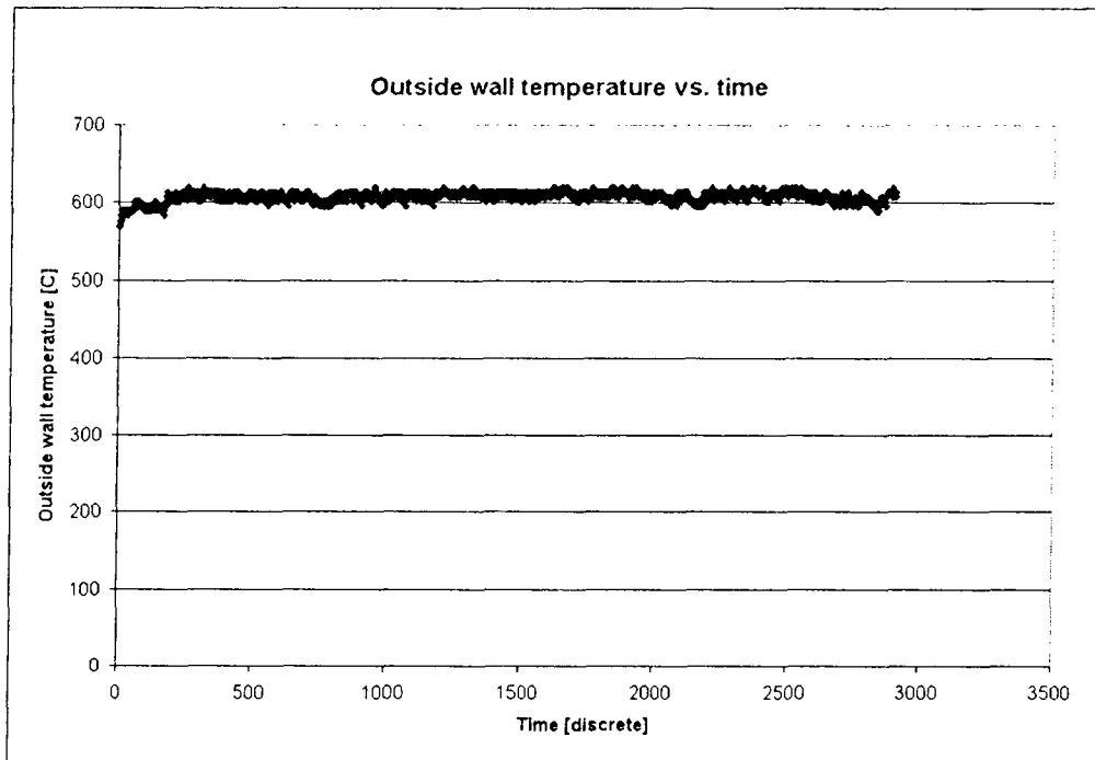
Figure 5-22: Outside wall temperature measured at 1,400 microns from the entrance during a stability test carried out at a critical pressure ratio \frac{P}{P_c} = 1.55 , a mass flow \dot{m} = 0.07 g/s and a heat flux q = 30 W/mm 2 .
