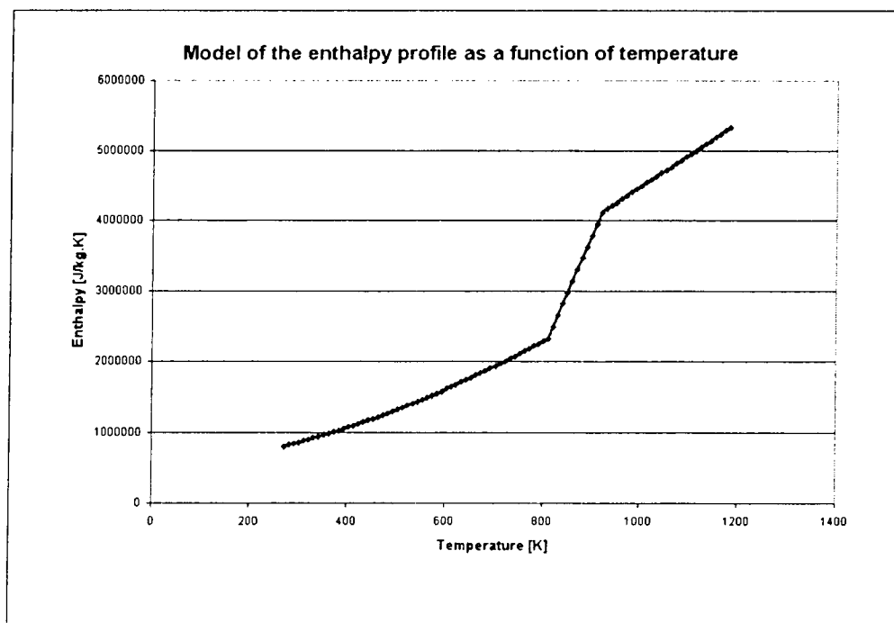
Figure 4-31: Model of JP7 enthalpy profile taking into account the endothermic decomposition. The model uses the assumptions presented in Table 4.1.
