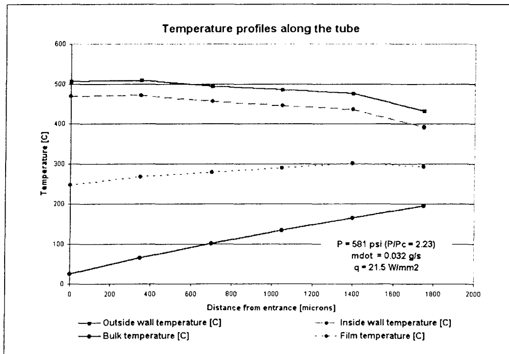
Figure 4-10: Outside wall temperature, inside wall temperature, bulk temperature and film temperature ( T_{film} = (T_i - T_{bulk})/2 ) as a function of the distance from the entrance of the tube. The outside wall temperature shows a flat profile along the tube.
