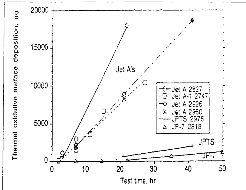
Figure 4-3: Surface deposition as a function of test time for 12 \text{ mL} \cdot \text{min}^{-1} tests [30].
