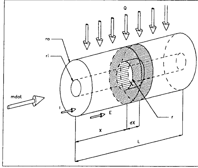
Figure 3-10: Schematic of the micro test section.
