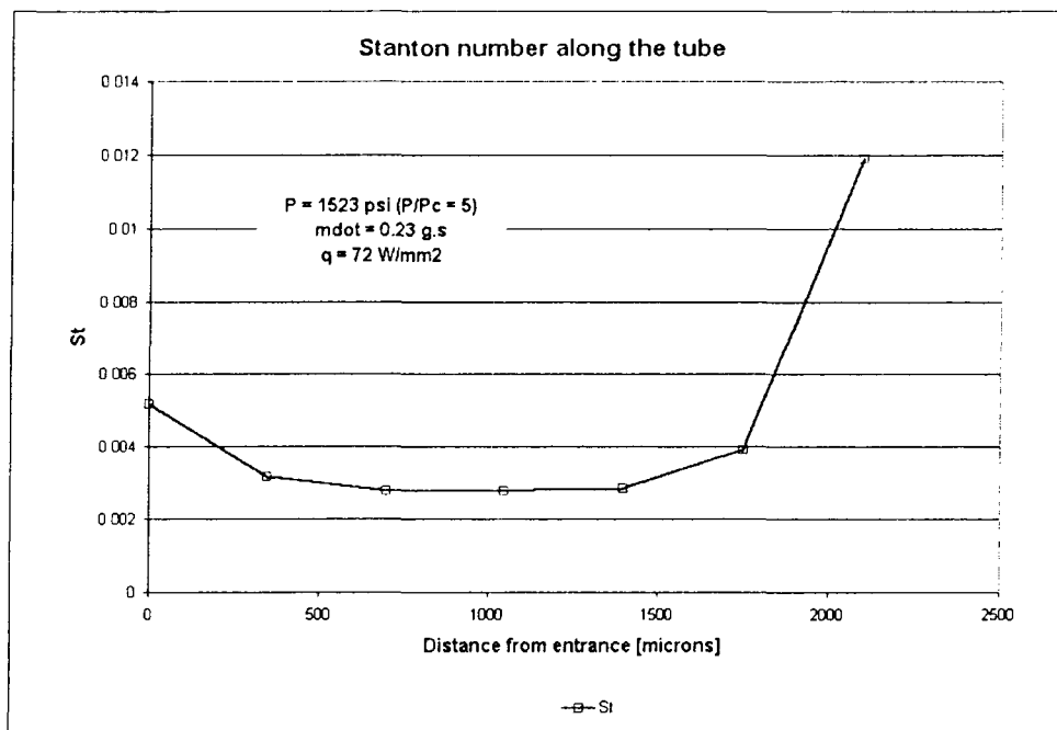
Figure 4-13: Stanton number along the tube for a test at 1,523 psi ( \frac{P}{P_c} = 5 ), a mass flow of 0.23 g/s and a heat flux of 72 W/mm 2 .
