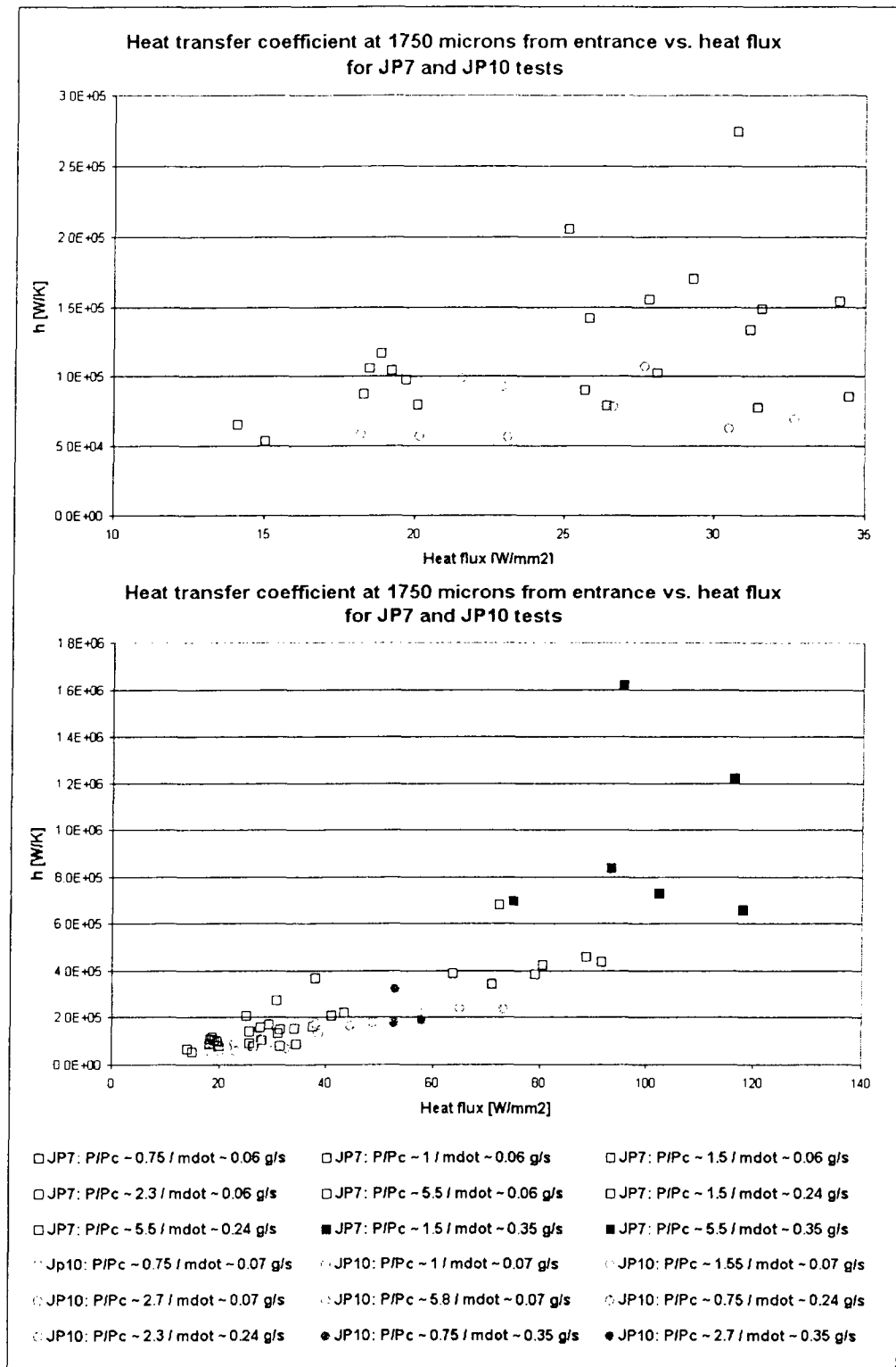
Figure 5-25: Heat transfer coefficients at 1,750 microns from the entrance as a function of heat flux for JP7 and JP10 tests.
