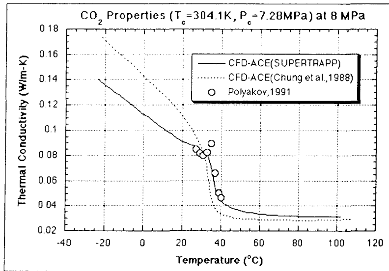
Figure 2-4: Thermal conductivity variation for CO_2 as a function of temperature near the critical point [11].
