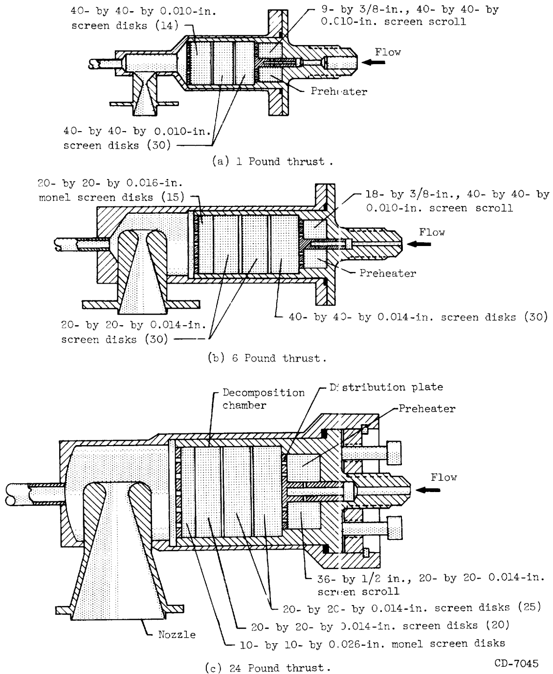
Figure 2. - Schematic of configuration B hydrogen peroxide thrust chambers.
