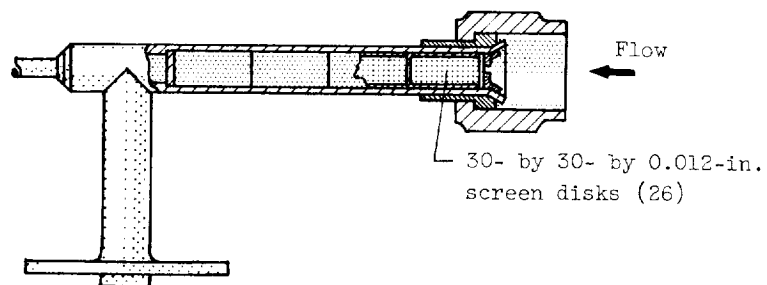
Figure 1. - Schematic of configuration A hydrogen peroxide thrust chambers.
