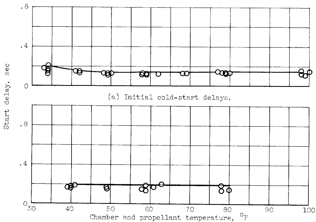
Figure 11. - Starting characteristics for hydrogen peroxide 6-pound-thrust chamber. Configuration B.
