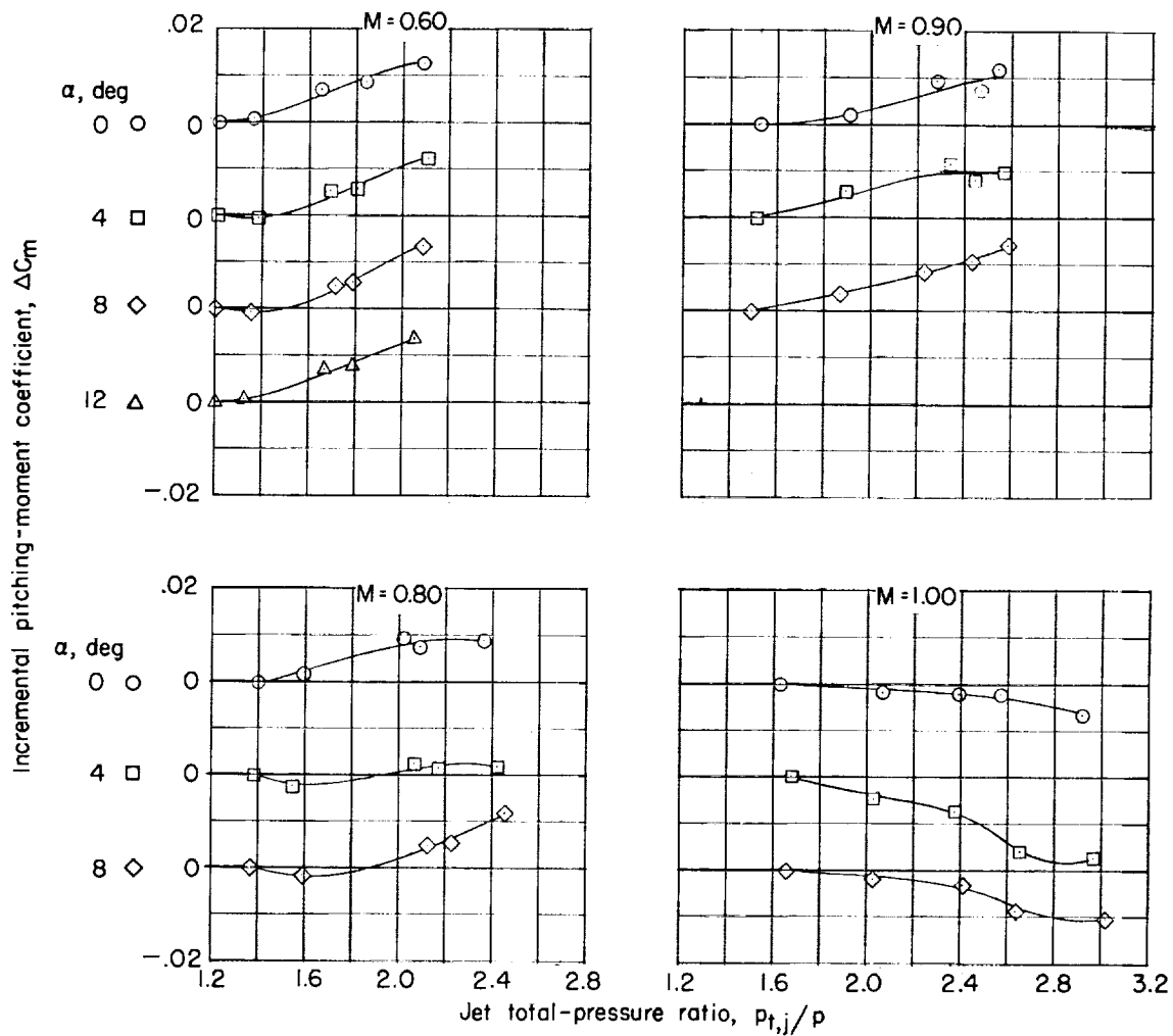
(c) Variation of incremental pitching-moment coefficient with jet total-pressure ratio.
