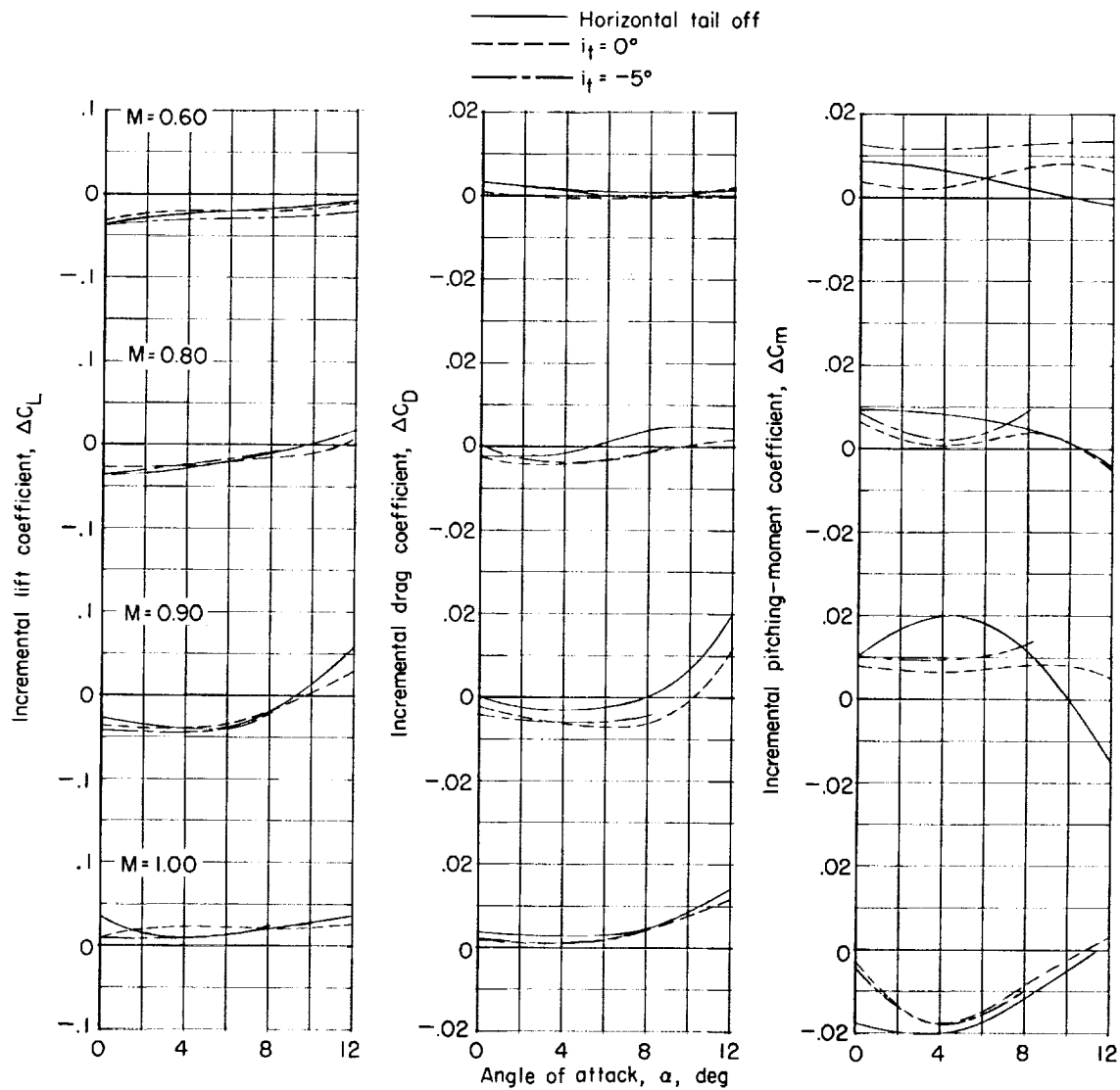
Figure 9.- Jet-induced incremental aerodynamic coefficients for three horizontal-tail configurations.
